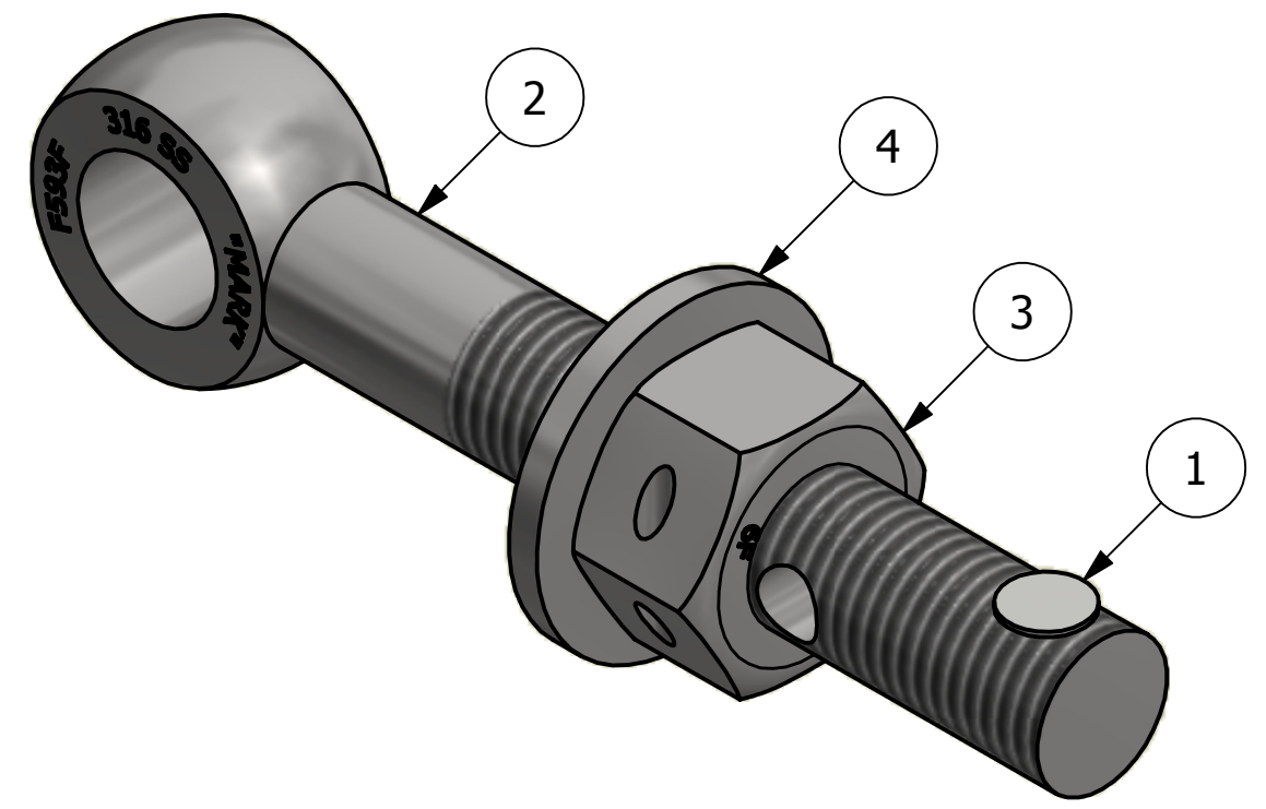
ISOMETRIC VIEW
